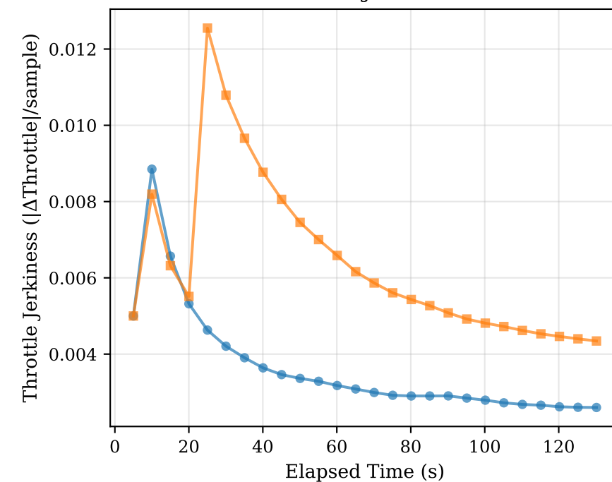
Throttle Jerkiness
