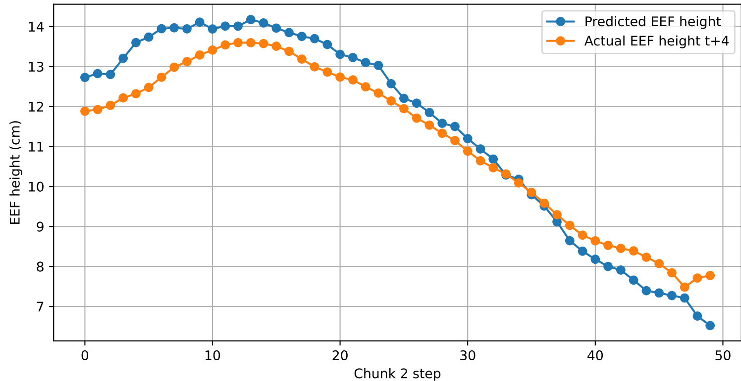
Episode 000009: predicted vs actual EEF height
