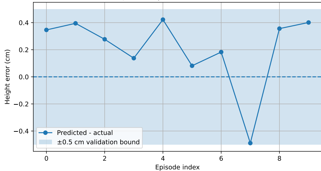
Residual EEF height error | mean=0.21 cm, max abs=0.49 cm
