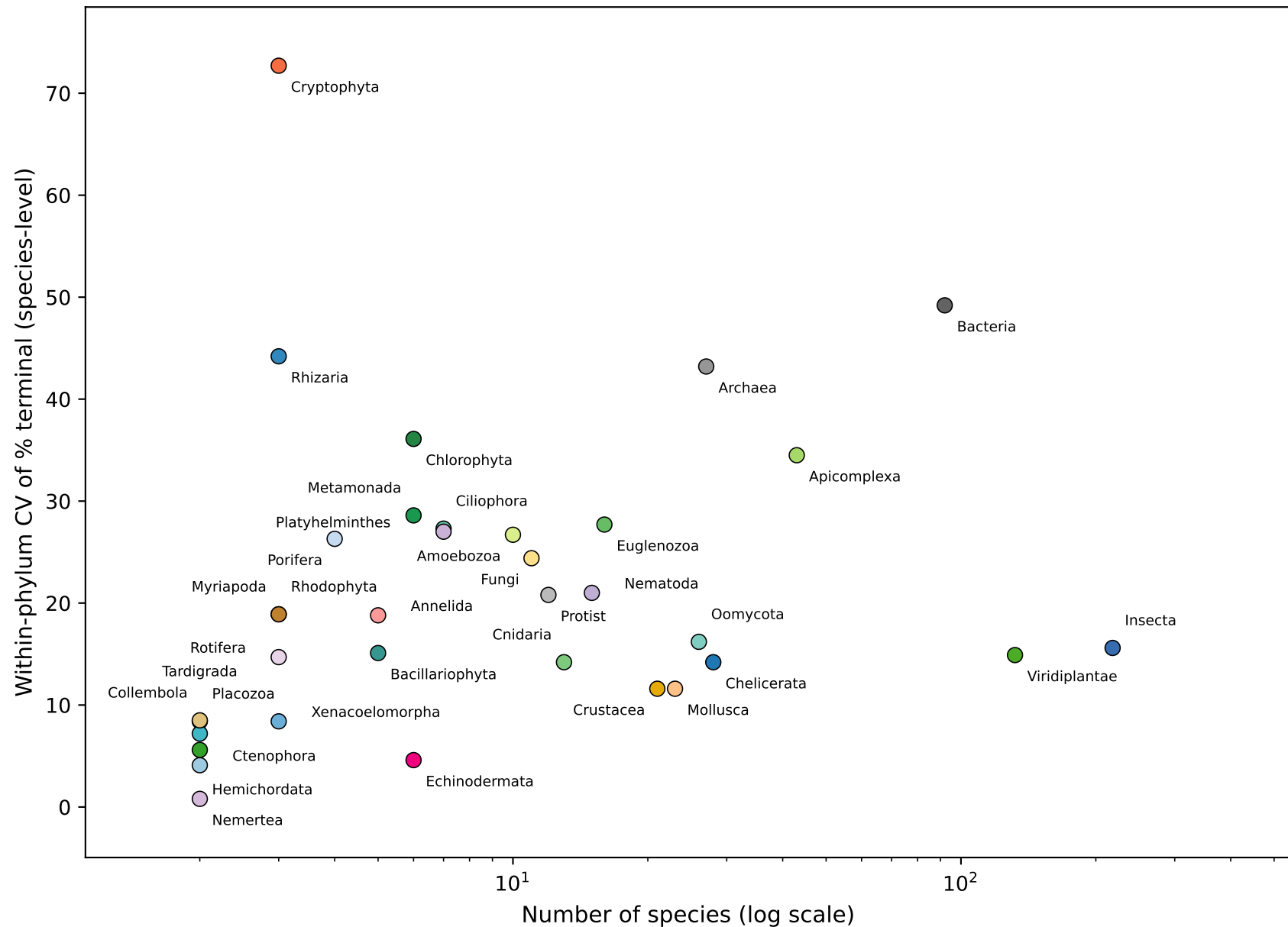
Within-phylum coefficient of variation vs. sampling depth (phyla/groups with n \geq 2 species)
