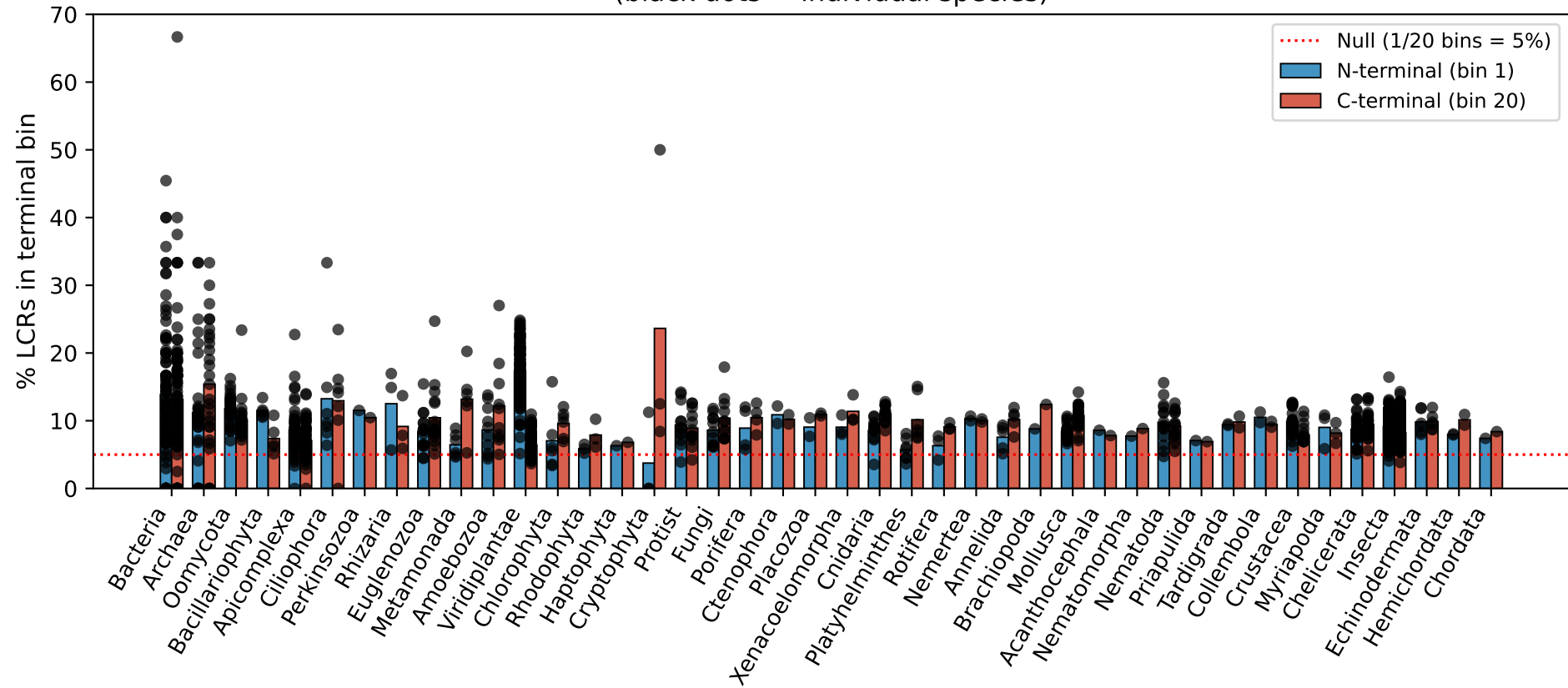
N-terminal vs C-terminal LCR enrichment per phylum (black dots = individual species)
