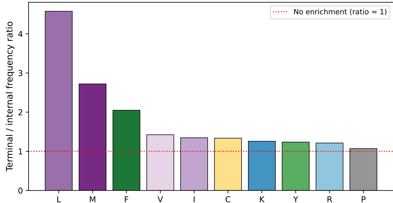
Amino acids enriched at protein termini (all species pooled)
