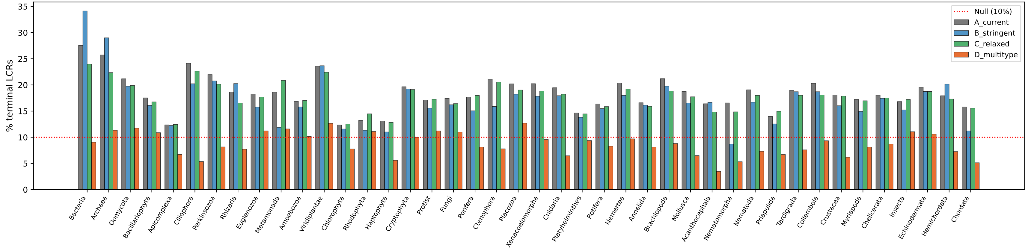
Sensitivity of terminal LCR enrichment to fLPS parameter choice A=current, B=stringent (len \geq 6, purity \geq 80%), C=relaxed (purity \geq 60%), D=MULTI-type
