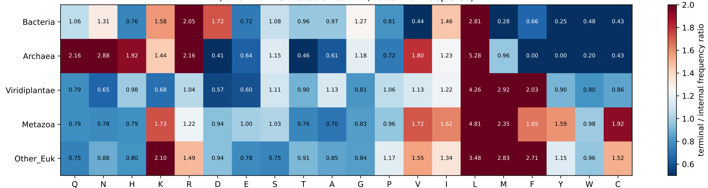
Amino acid enrichment at termini by domain (ratio > 1 = enriched at termini; ratio < 1 = depleted)
