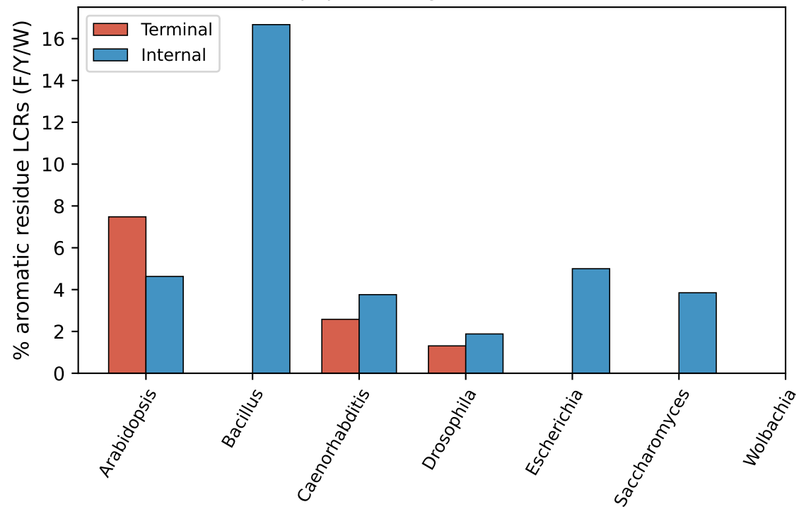
Aromatic LCR fraction at termini vs internal (pi-pi stacking drives LLPS)
