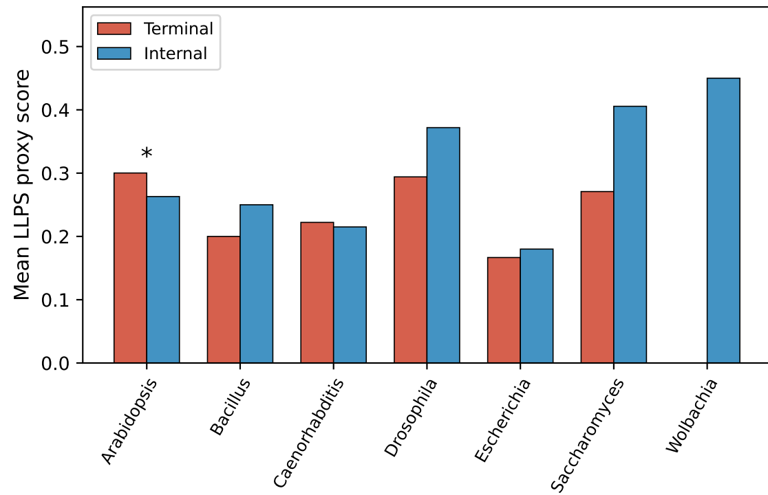
Composition-based LLPS propensity terminal vs internal LCRs
