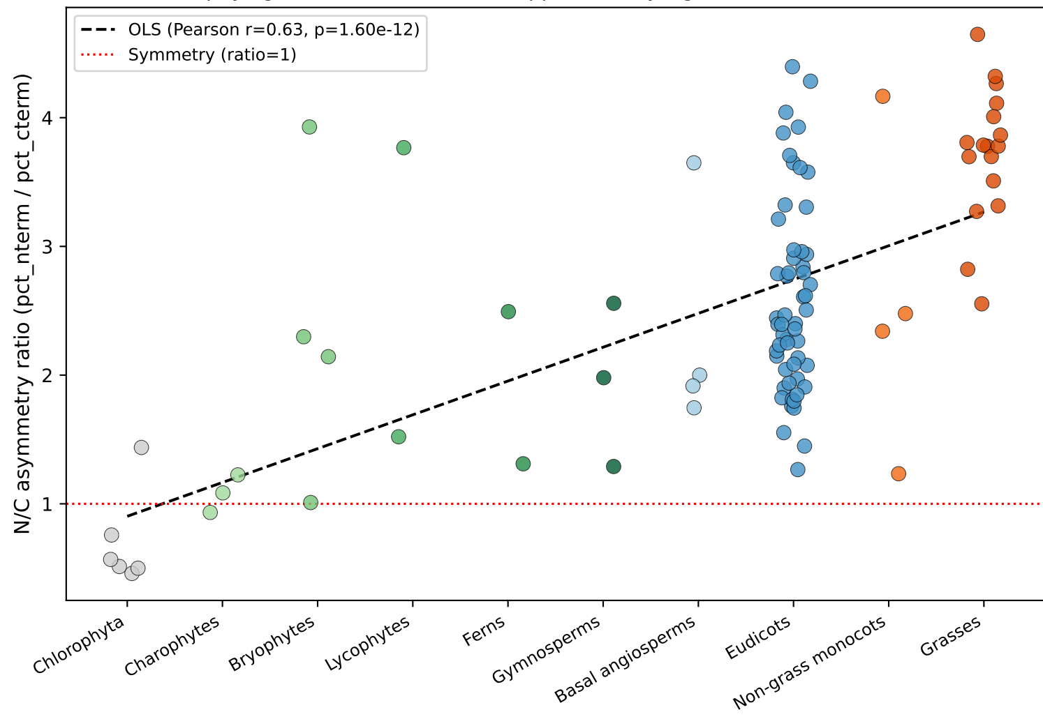
Viridiplantae N/C asymmetry ratio across evolutionary tiers (n=100) (non-phylogenetic OLS trend; see Supplementary Figure 7 for PGLS correction)
