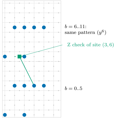
Figure 6: A weight-12 logical X error (coset id 128). Blue: flipped L qubits. Green: the three L legs of the Z check of site (3,6) (moves x^{-1}, x^{-2} to the edges left and right of it, y^{-3} far down; the dashed leg ends on an unflipped qubit). It overlaps the error on two qubits, so it does not fire. All 18 Z checks that touch the pattern overlap it on exactly two qubits, so the syndrome is zero.
