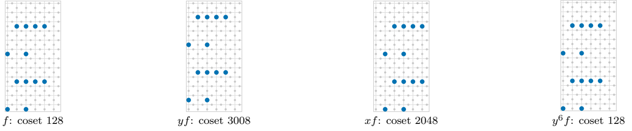
Figure 7: One orbit. Shifting the logical of fig. 6 by y or by x gives other cosets; shifting by y^6 gives the same pattern back, because f = (1 + y^6)(\dots) . Of the 72 shifts, pairs give the same coset, so this orbit has 72/2 = 36 cosets.
