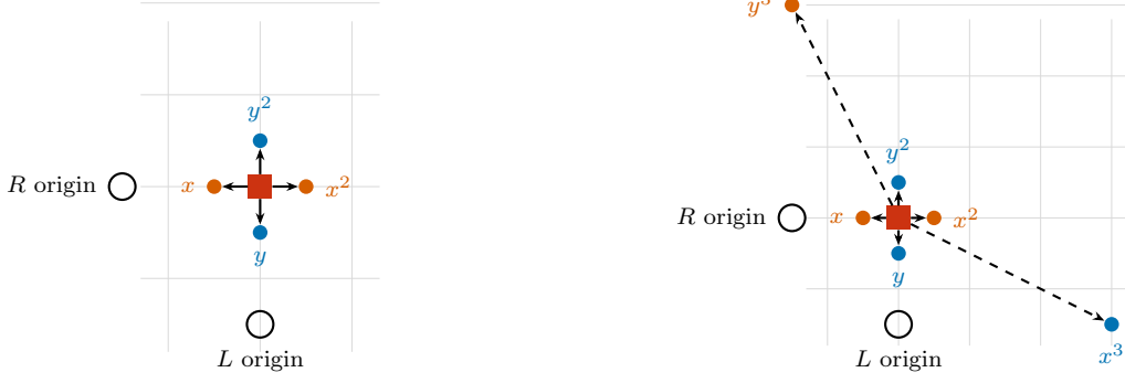
(a) Toric code, A = y + y^2 , B = x + x^2 : the four nearest edges. (b) Gross code, A = (y + y^2) + x^3 , B = (x + x^2) + y^3 : the same four, plus two long legs (dashed).
