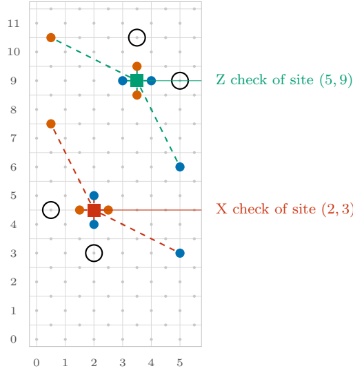
Figure 3: The whole gross code ( x right, y up; tick labels are a and b ) with two checks drawn. Each touches the four edges around it (solid) and two distant qubits (dashed); black rings mark the origins L(a,b) , R(a,b) of its site. The X check uses A from the L origin and B from the R origin; the Z check uses the reversed moves, B^{-1} on L and A^{-1} on R . Checks near the border have legs that wrap around the torus.
