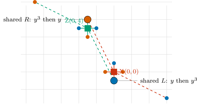
Figure 4: The X check at (0,0) and the Z check at (0,4) share exactly two qubits, one L and one R . Their offset y^4 = y \cdot y^3 can be split as “ y \in A then y^3 \in B ” (meeting on L : a local leg of X, a long leg of Z) or “ y^3 \in B then y \in A ” (meeting on R : a long leg of X, a local leg of Z).
