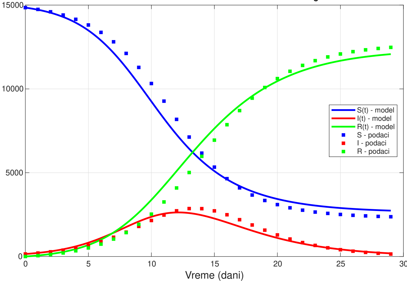
SIR model - Osn. sc. a=0.710 , r=0.336 , R_0=2.08
