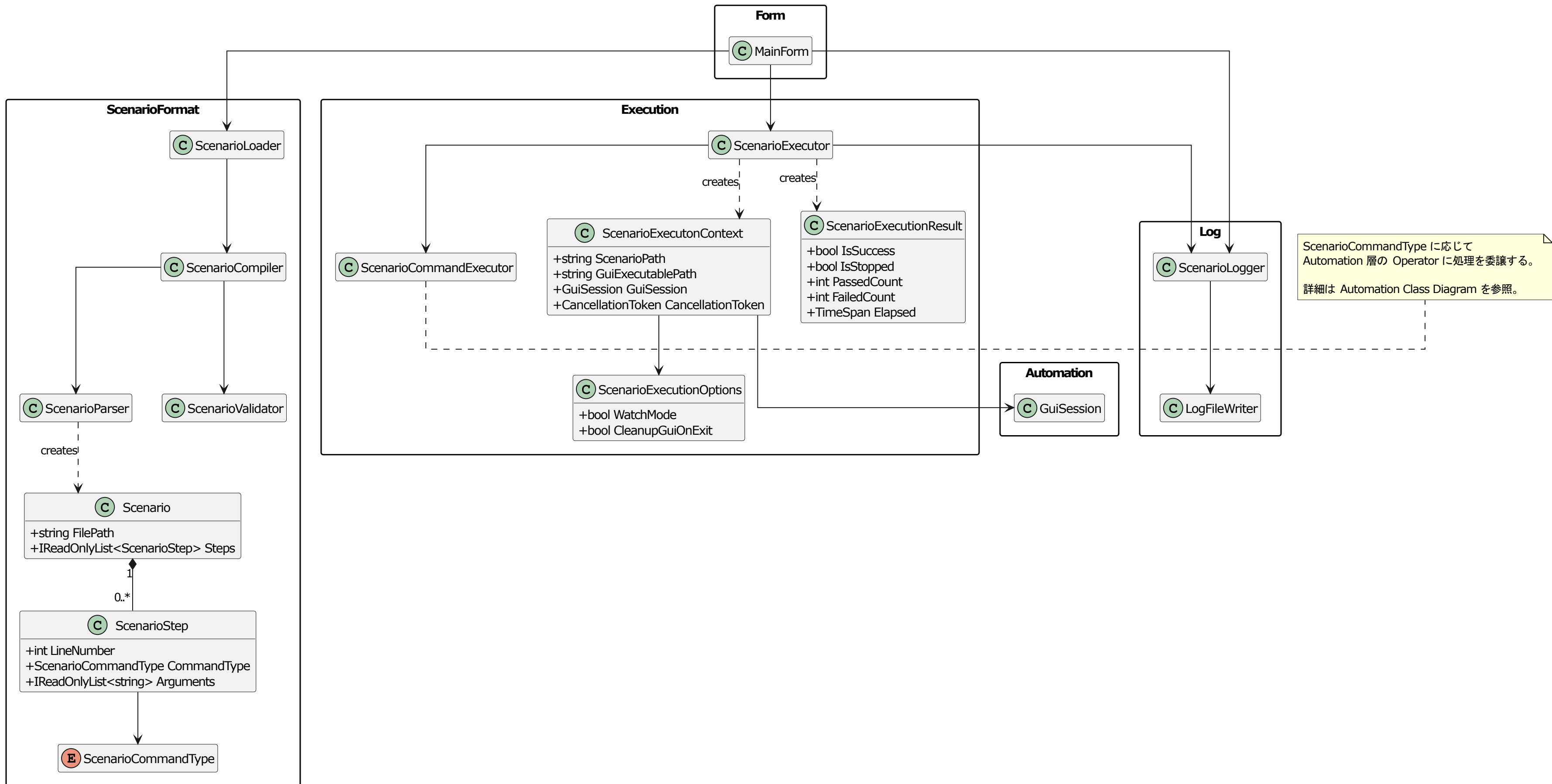
ShikigamiApp Scenario Runner - Class Diagram
