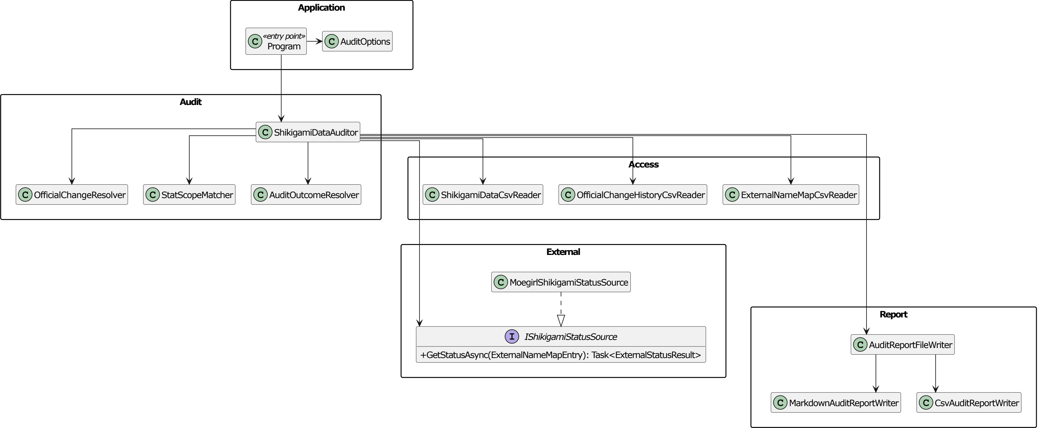
Shikigami Data Auditor - Class Diagram
