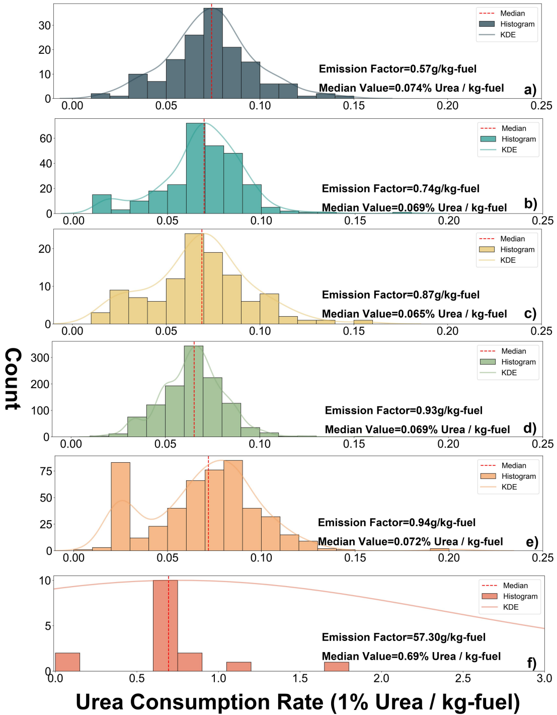
3 Figure 7. Distribution of Urea Consumption Rates Among Identical Vehicle Models. The red line 4 indicates the median urea consumption rate of the corresponding vehicle, and the KDE plot (Kernel 5 Density Estimation) illustrates the smoothed distribution.
