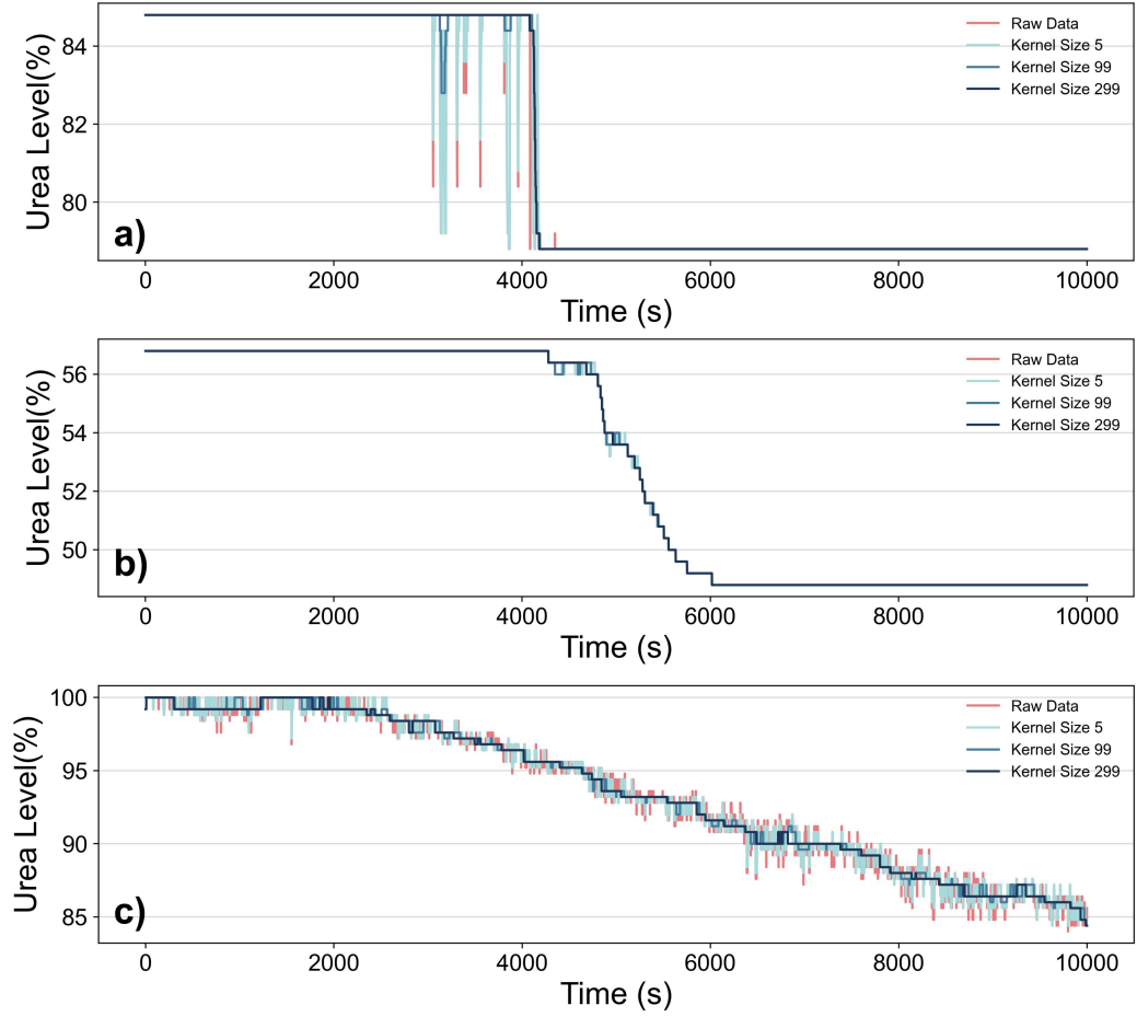
1 2 Figure 3. Performance of Medium Filters with Varying Kernel Sizes across Different Types of Urea 3 Level Decline. a) Threshold-triggered type with fluctuations around two discrete levels; b) 4 Threshold-triggered type with a gradual decline after reaching a certain threshold; c) Sensitive type 5 with continuous and smooth decline behavior.
