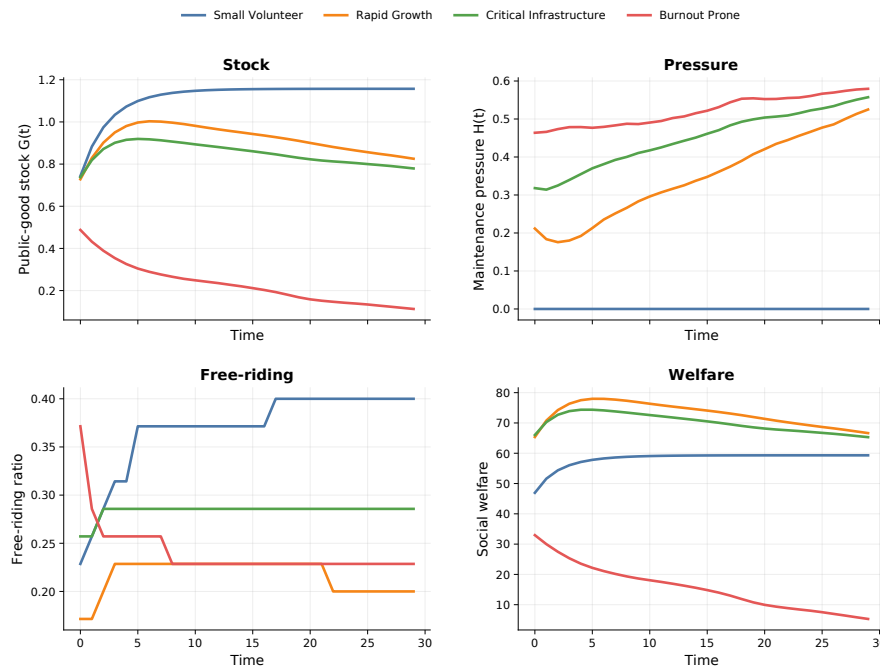
Figure 7: Baseline dynamic behavior under synthetic scenarios. The panels compare stock, maintenance pressure, free-riding ratio, and welfare under the baseline Nash-style simulation.
