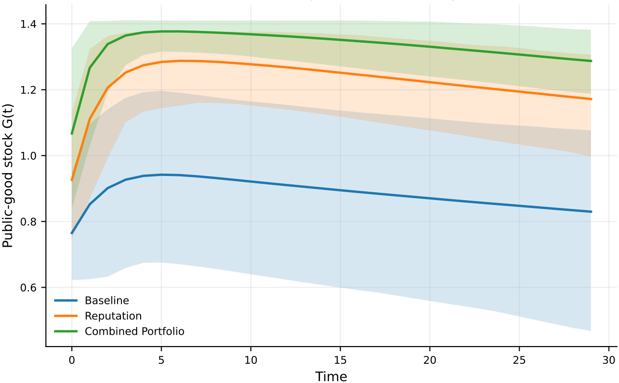
Monte Carlo Uncertainty Band for Public-good Stock
