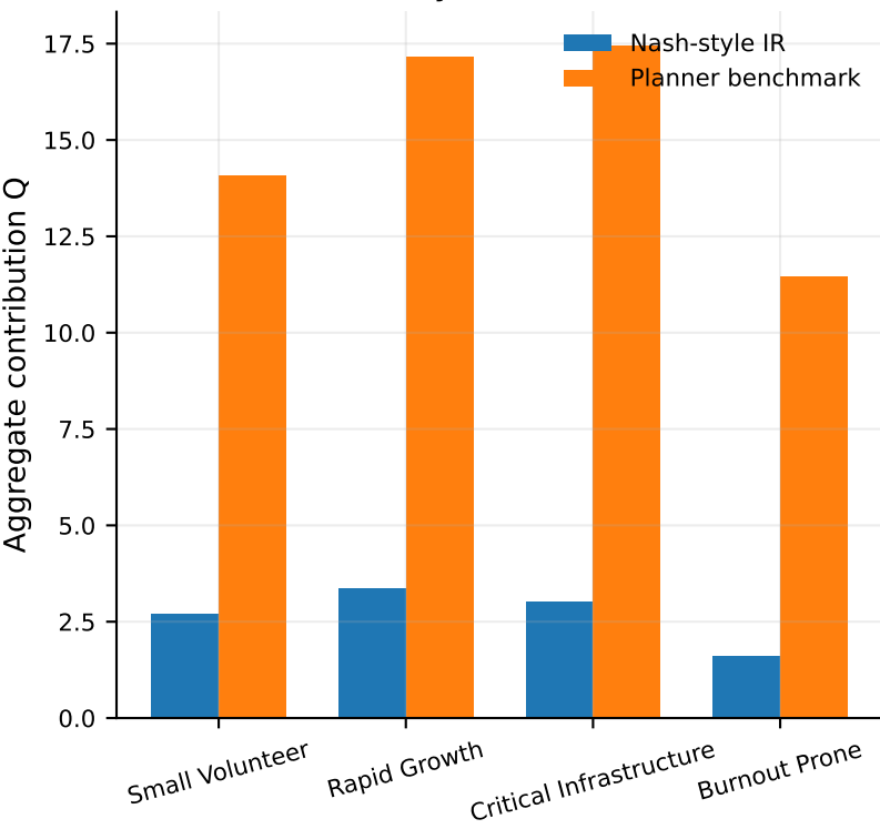
Contribution: Nash-style IR vs Planner Benchmark
