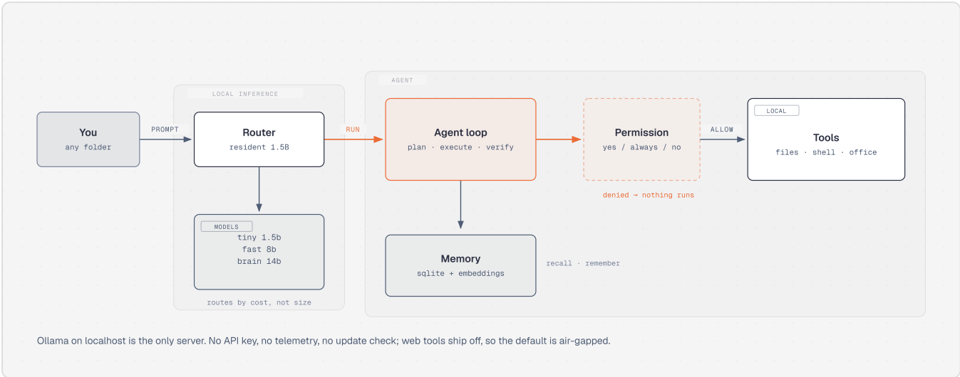
Fig. 1 – end to end. Ollama on localhost is the only server.
