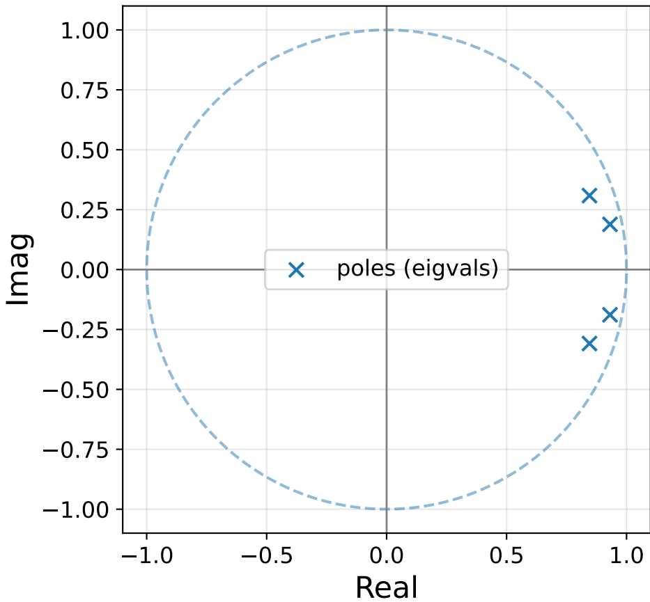
Discrete-time Poles (A)
