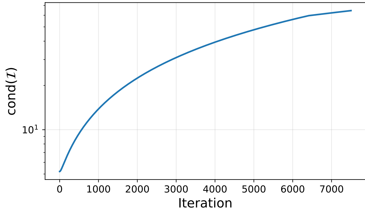
Fisher Information Condition Number (4D)
