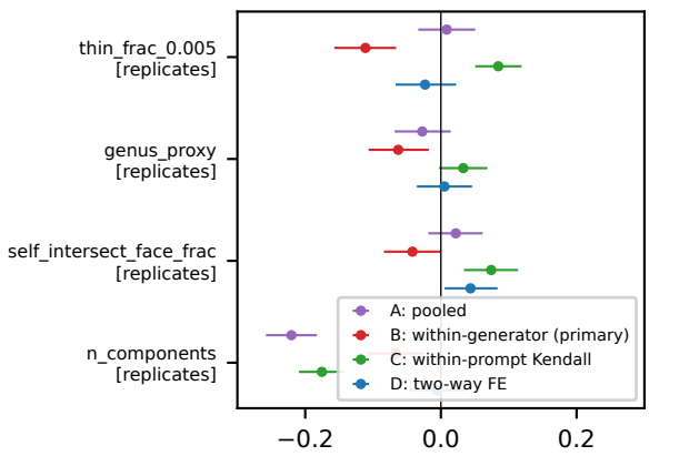
geometry_score (primary)
