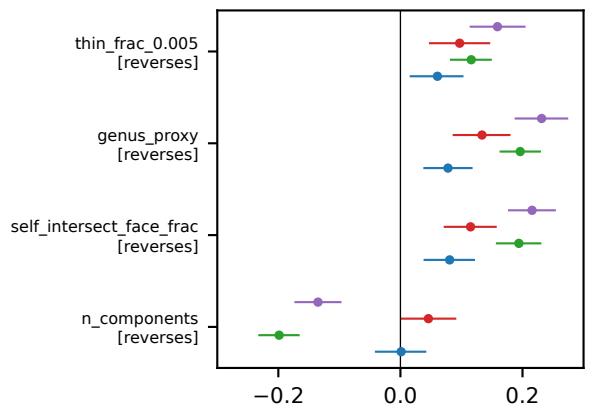
geo_detail_score (secondary)
