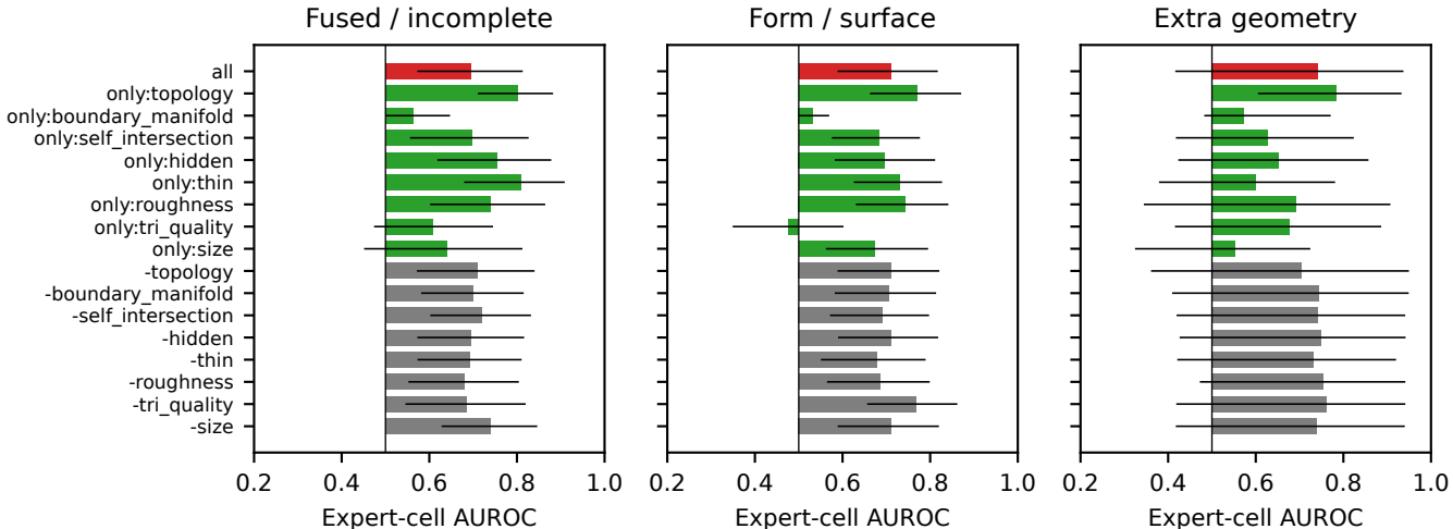
Feature-family ablation (silver-trained; test-set observation, not used for model selection)
