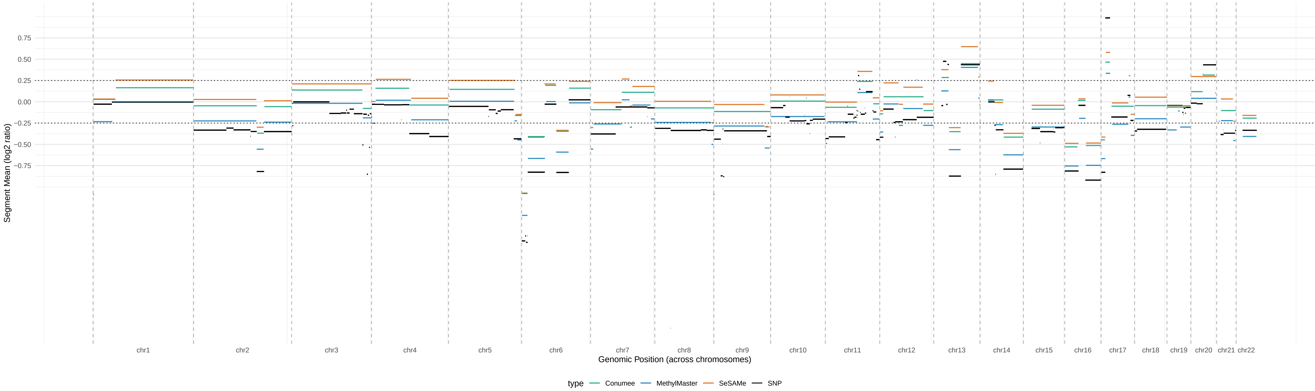
CNV Segments – LMS11 (LMS, 1e+06 bp bins)
