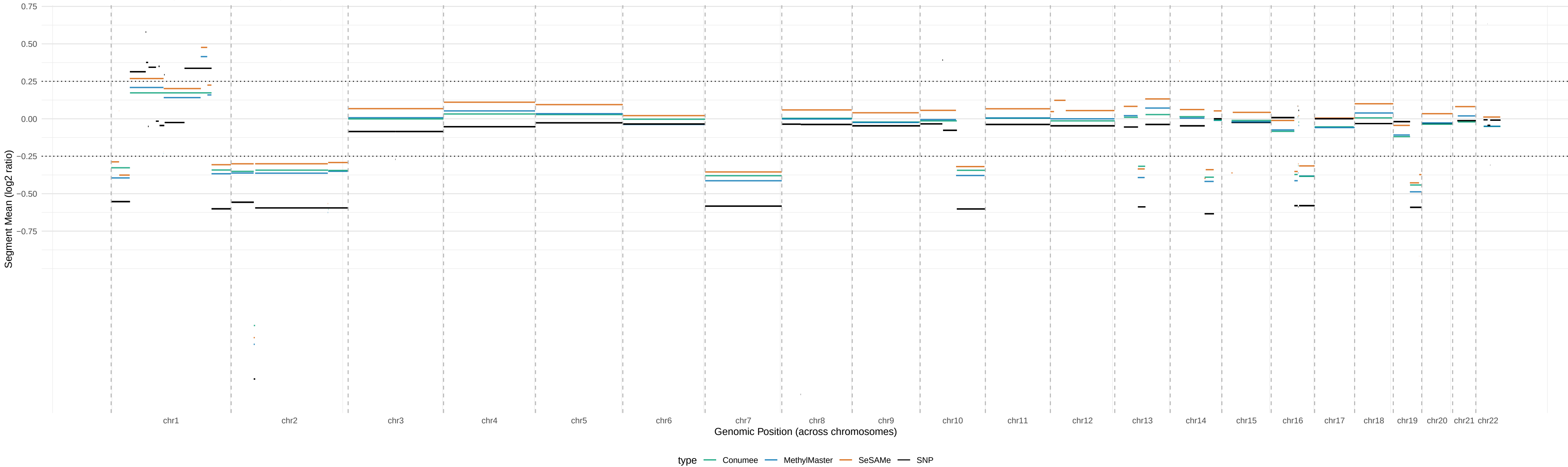
CNV Segments – LMS2 (LMS, 10000 bp bins)
