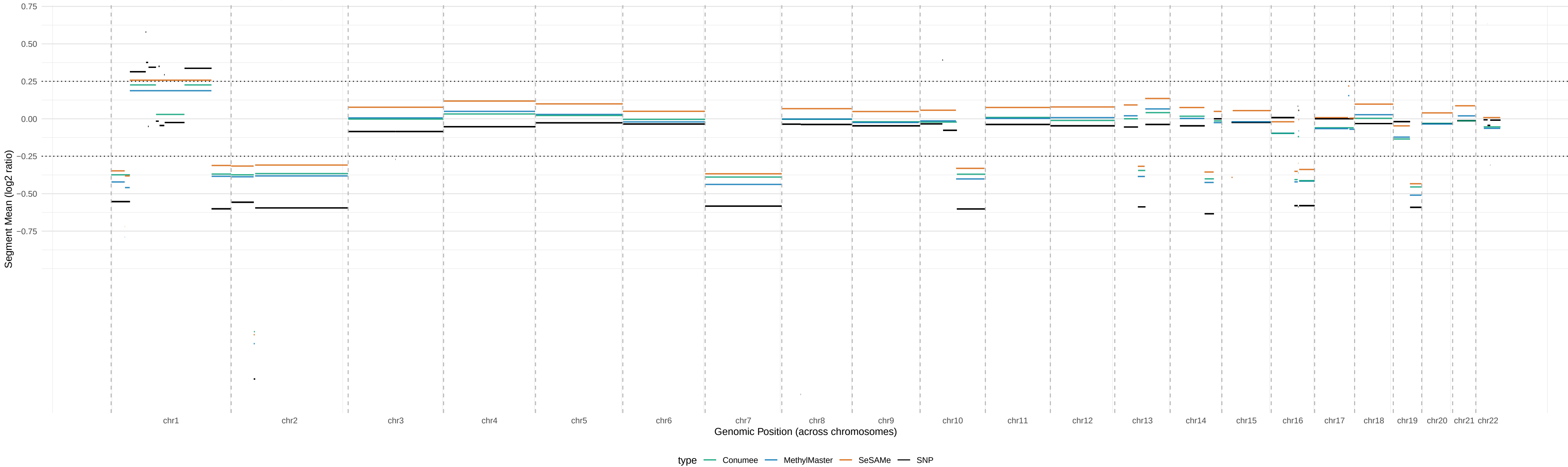
CNV Segments – LMS2 (LMS, 1e+05 bp bins)
