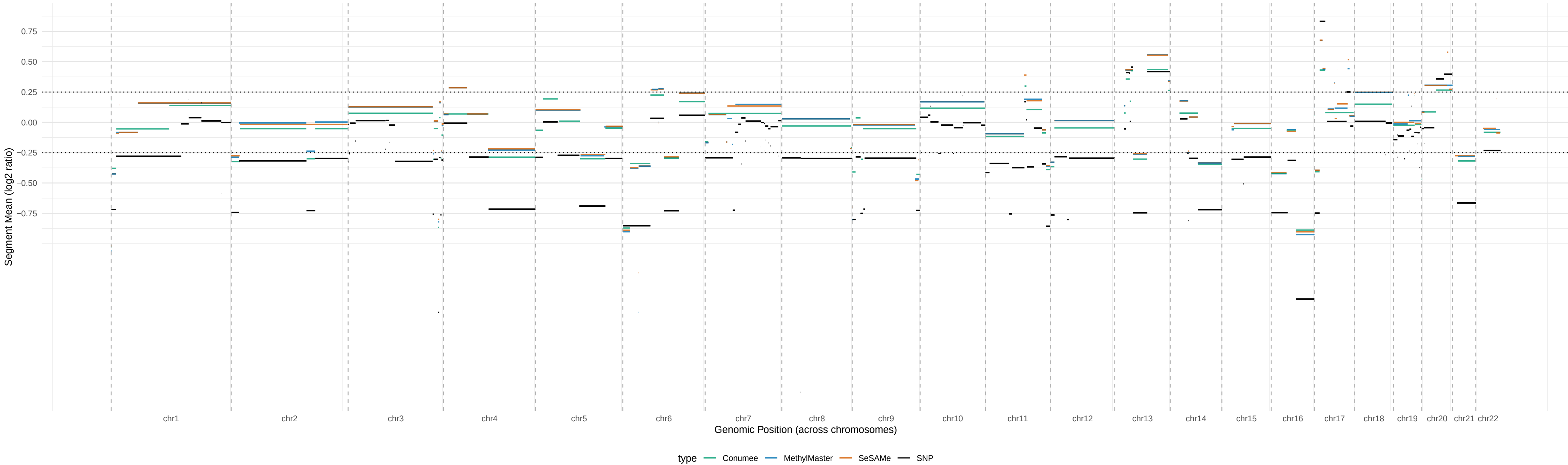
CNV Segments – LMS3 (LMS, 10000 bp bins)
