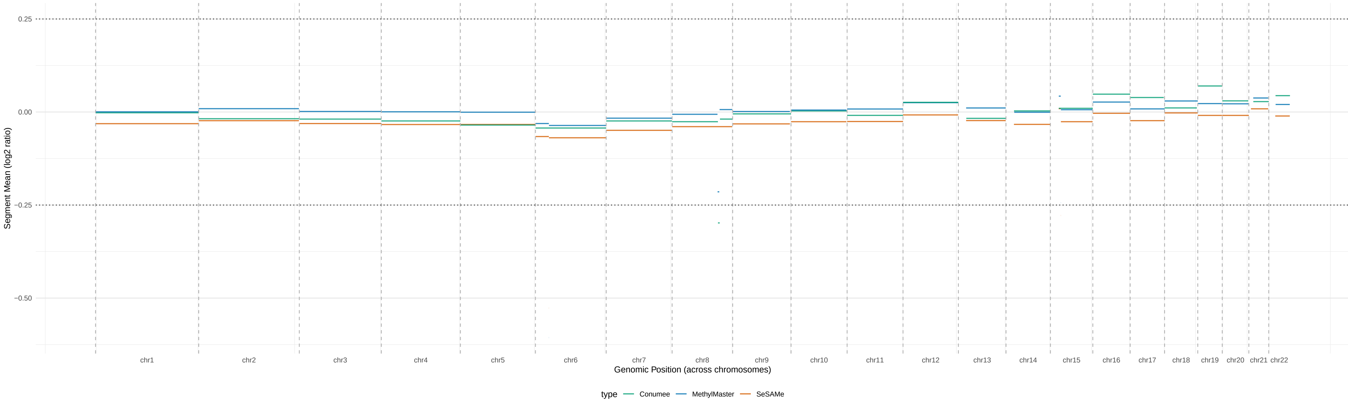
CNV Segments – NORM4 (Normal, 50000 bp bins)
