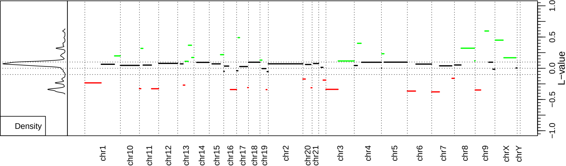
Sample:: 205243940046_R04C01
