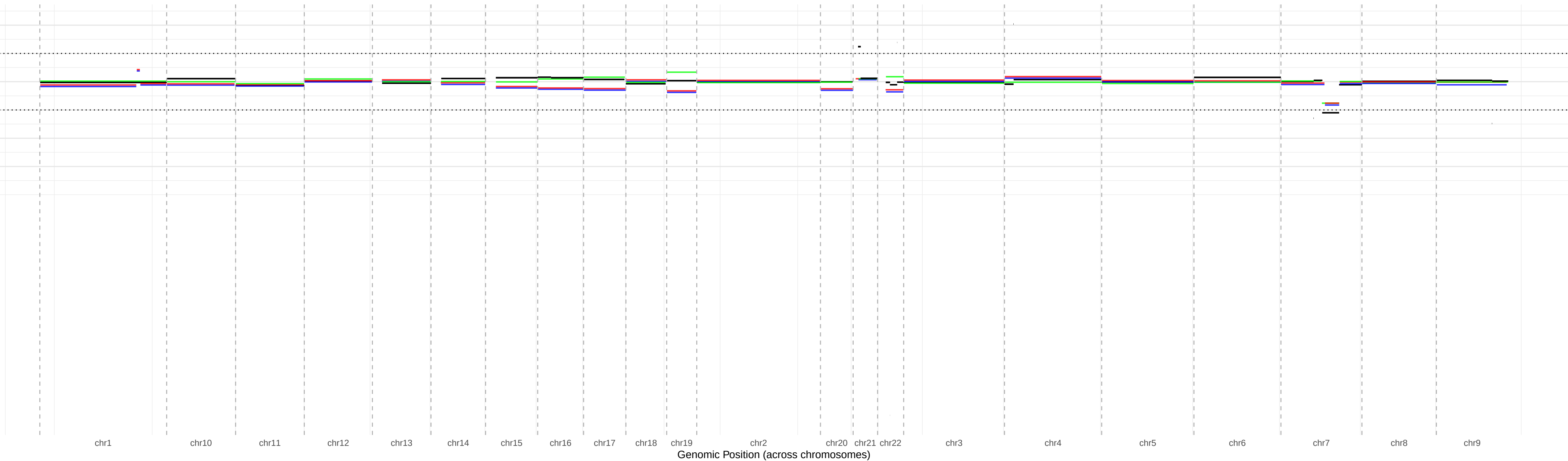
CNV Segments Across Genome
