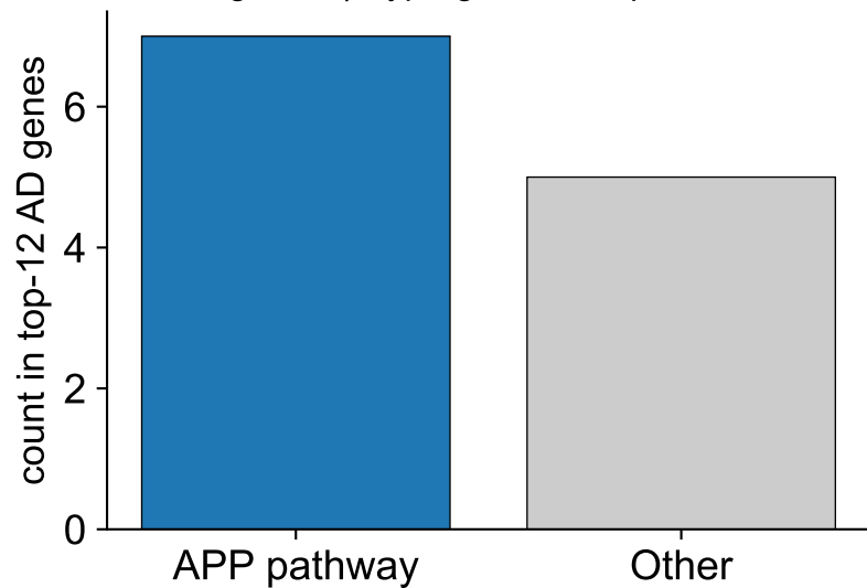
Fig 3B-2 | Hypergeometric: p=0.0000
