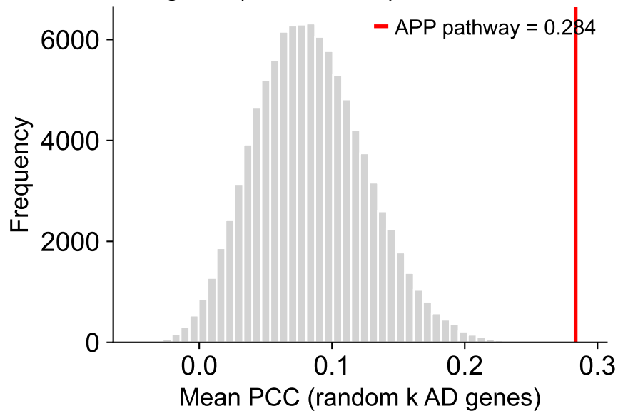
Fig 3B-1 | Permutation: p=1.0e-05 , z=4.79
