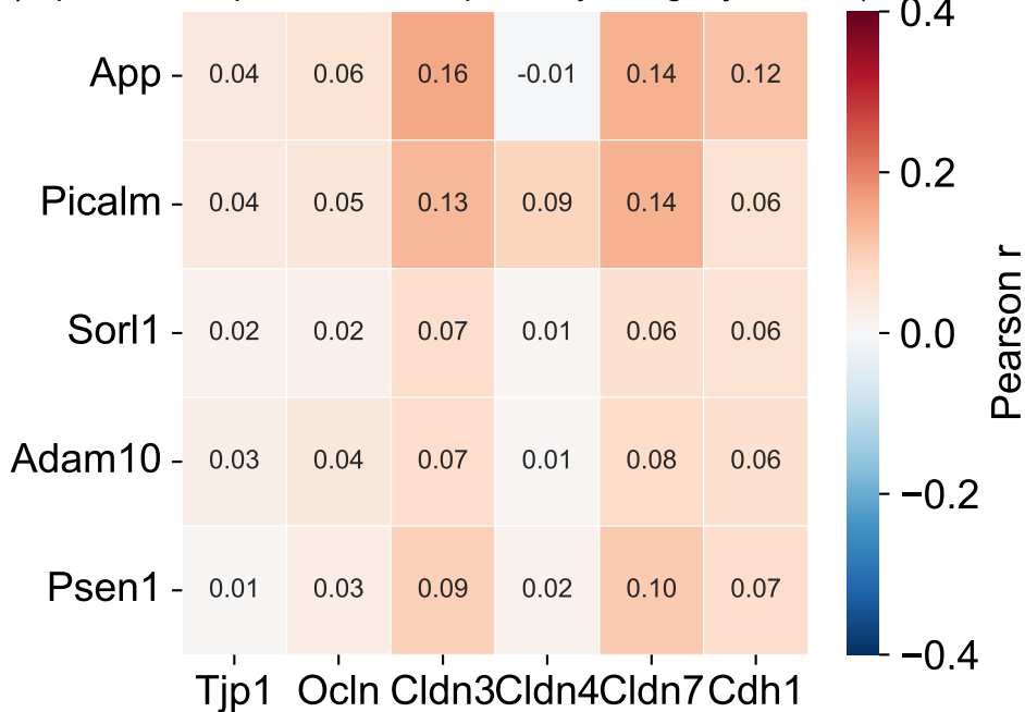
Fig 3D | Spatial co-expression: APP-pathway vs tight-junction (Colon CTRL1)
