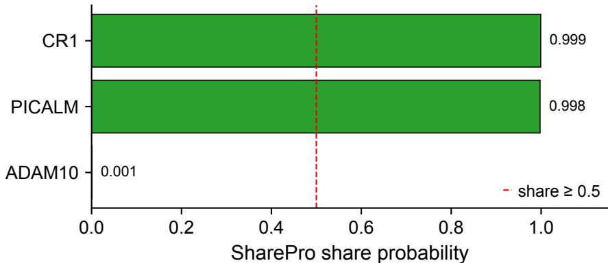
Fig 4C | Multi-causal coloc — SharePro rescues PICALM
