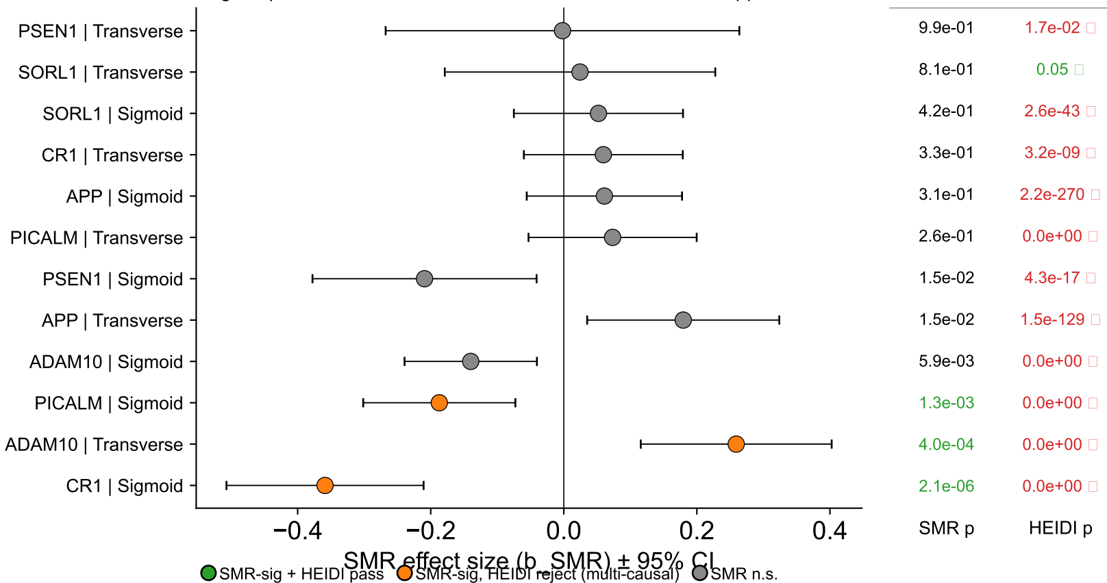
Fig 4D | SMR + HEIDI — multi-causal architectures inflate apparent SMR
