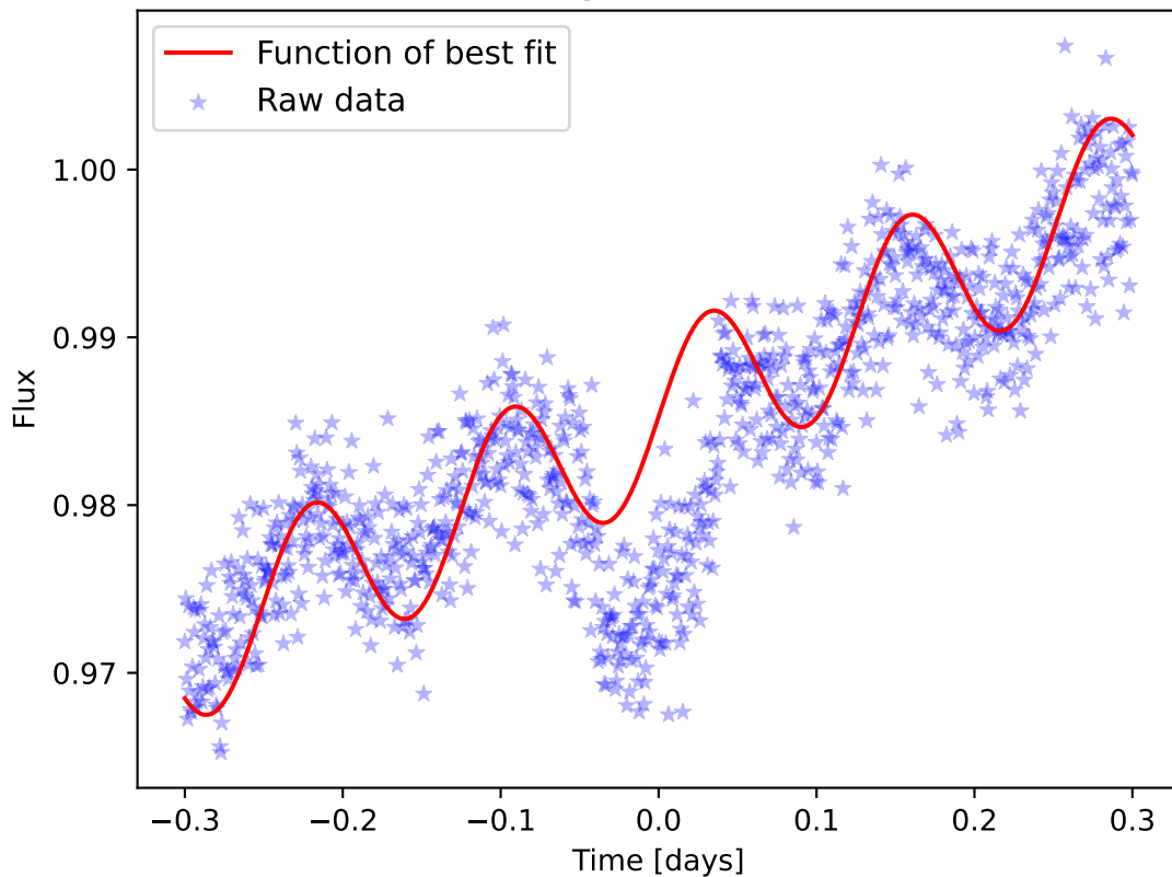
Planet Light Curve Best Fit
