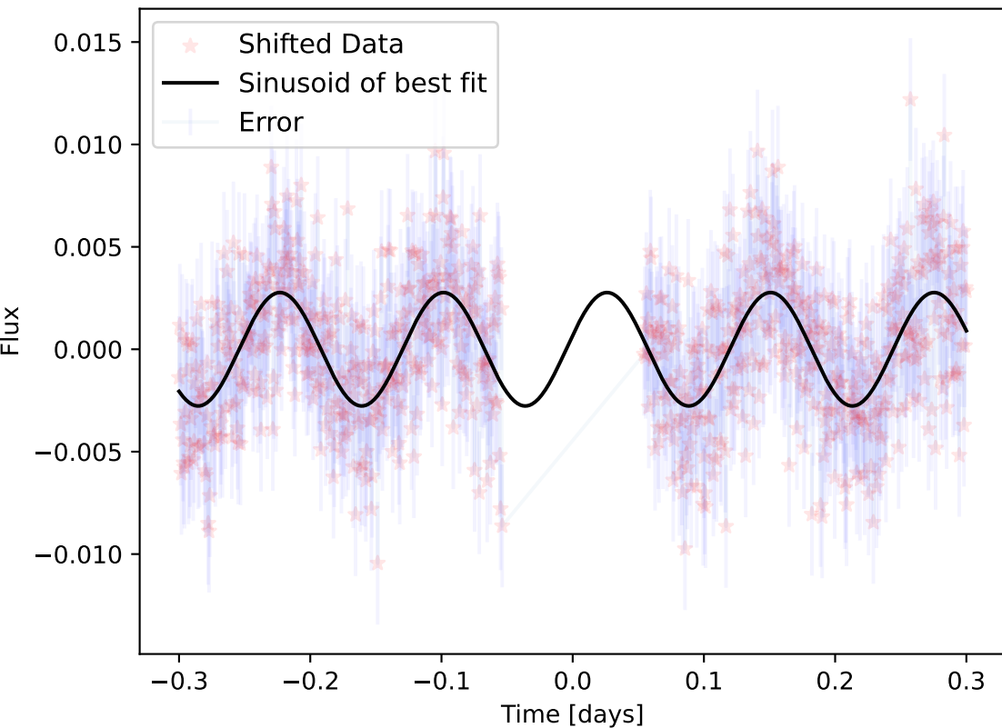
Best Fit of Stellar Flux, Shifted To Sinusoid, With Cut Data
