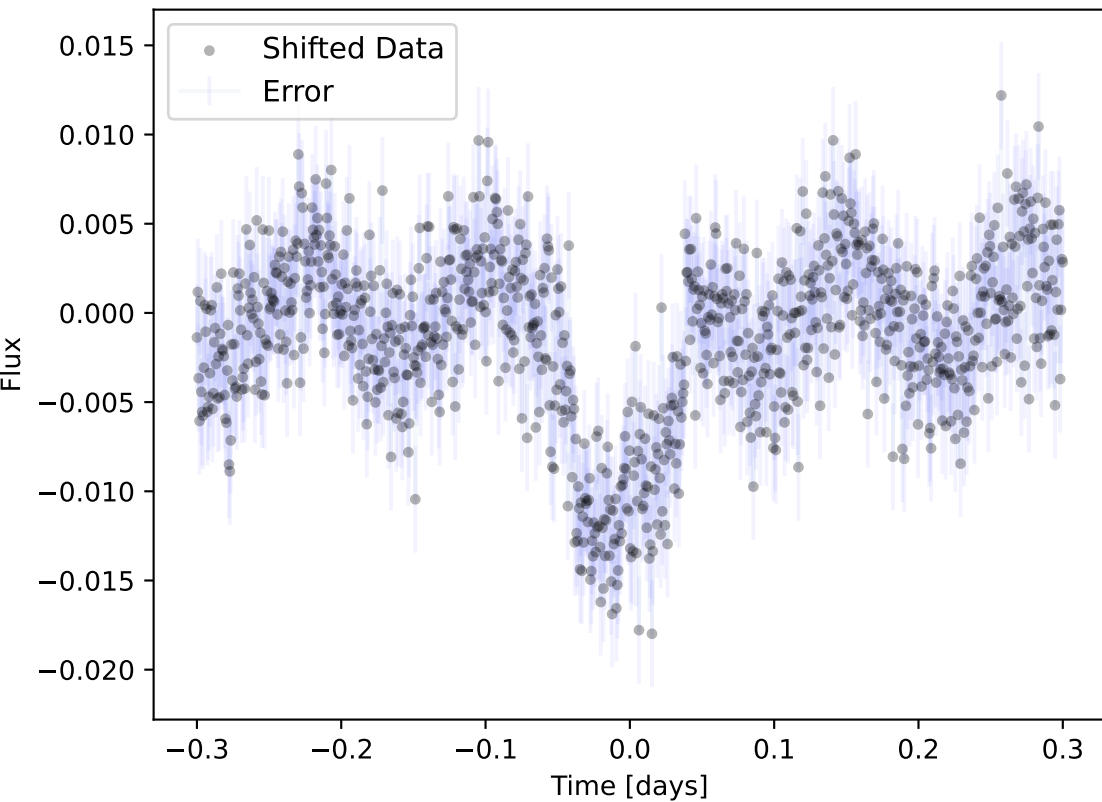
Stellar Flux Over Time, Shifted
