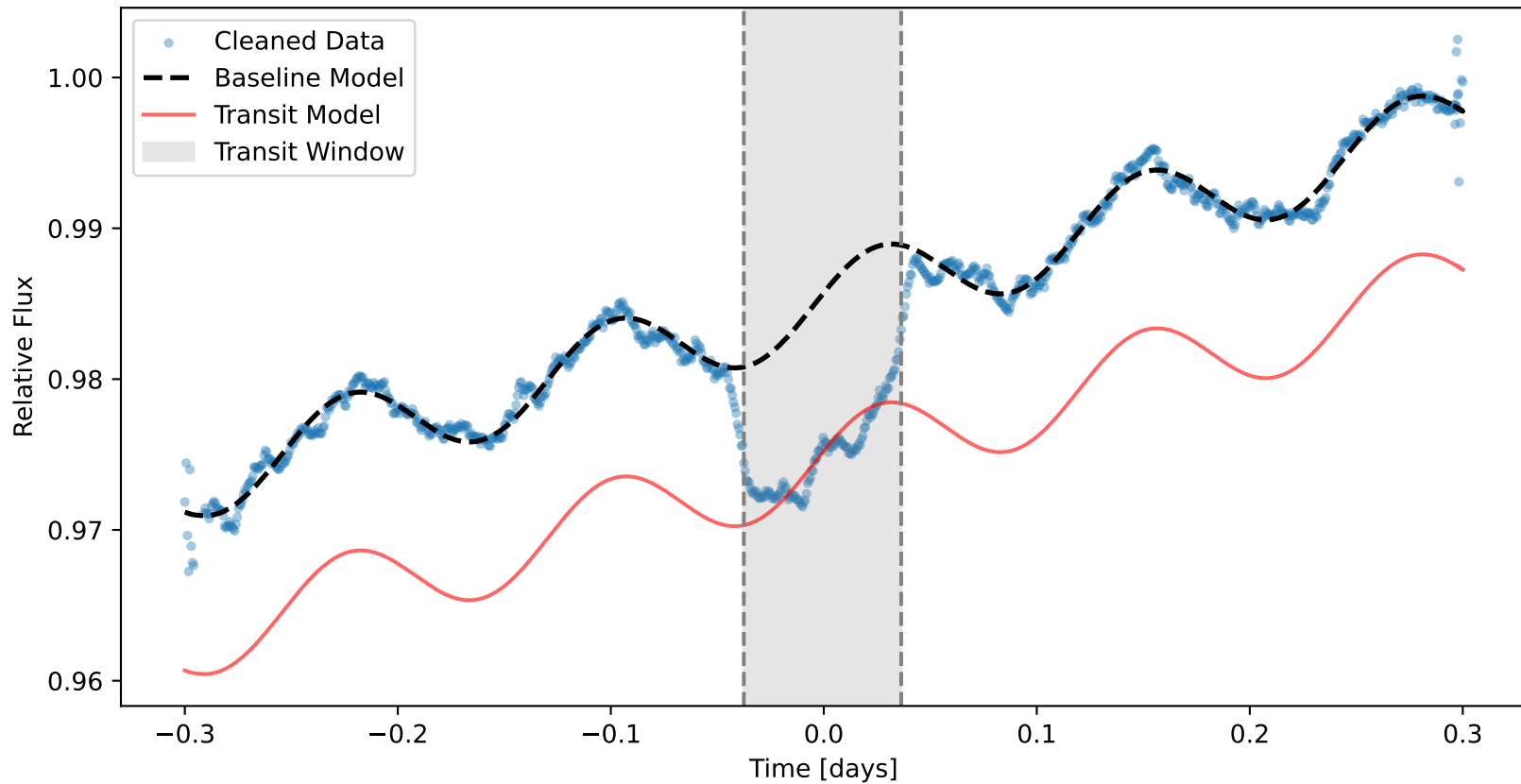
Exoplanet Transit Depth and Duration
