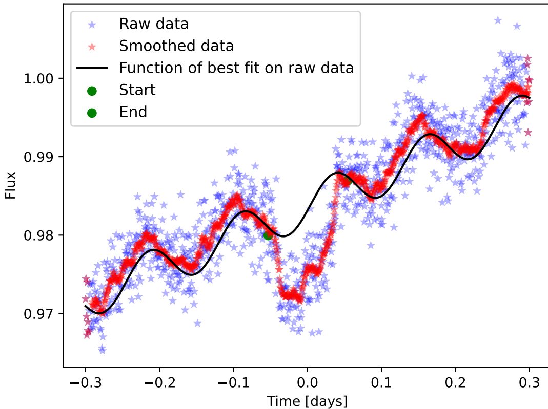
Planet Light Curve Best Fit Smoothed With Moving Mean
