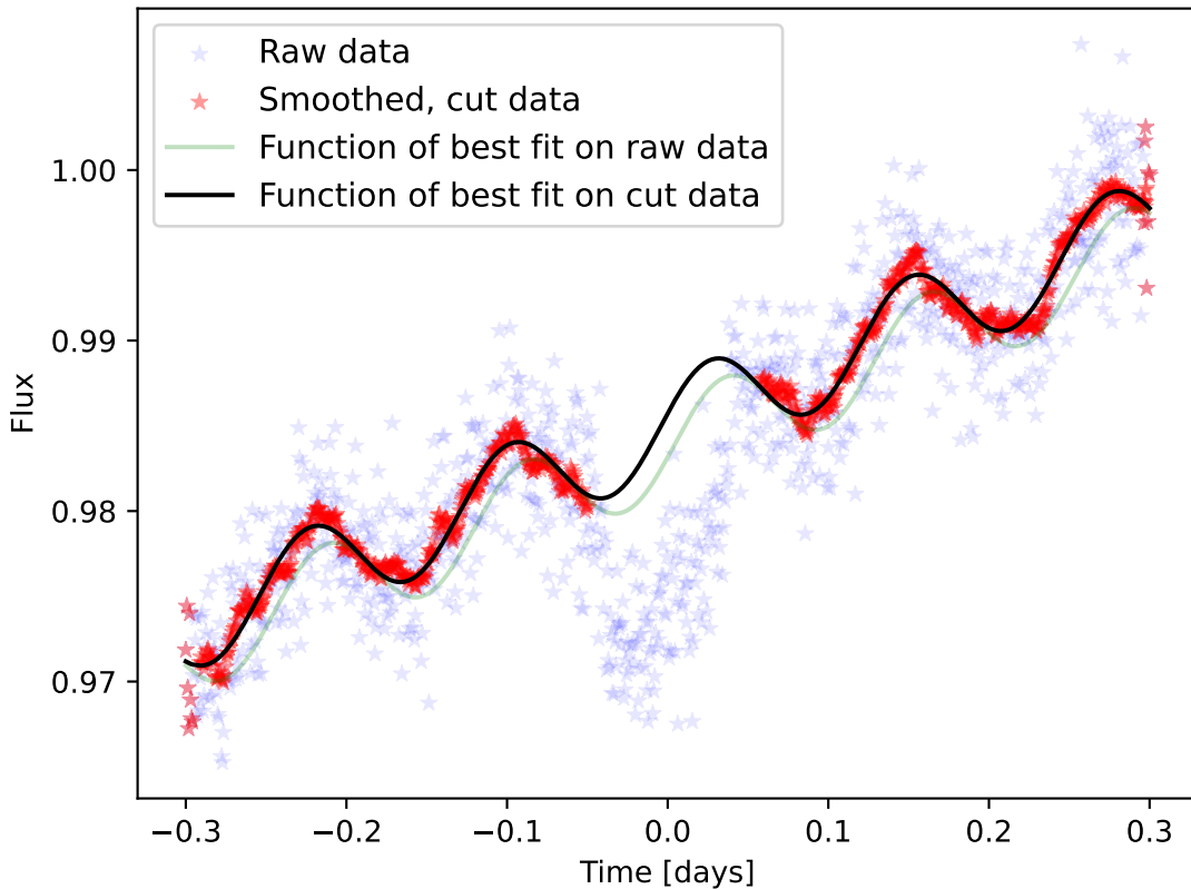
Planet Light Curve Best Fit Smoothed With Moving Mean and Cleaned Data
