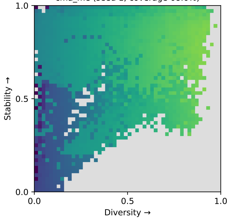
cma_me (seed 1, coverage 68.6%)
