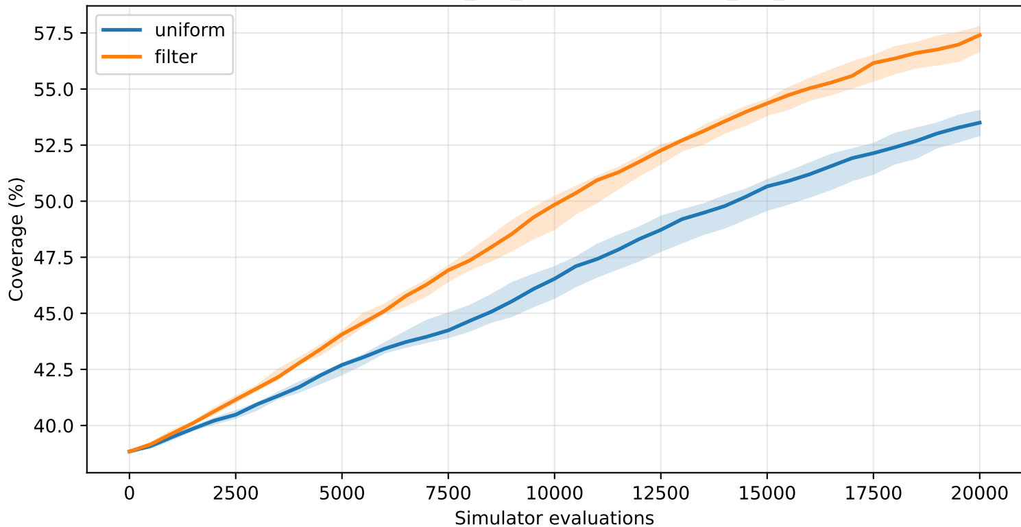
H2 (after-generation): genetic_me_uniform vs genetic_me_filter (n=10, IQR)
