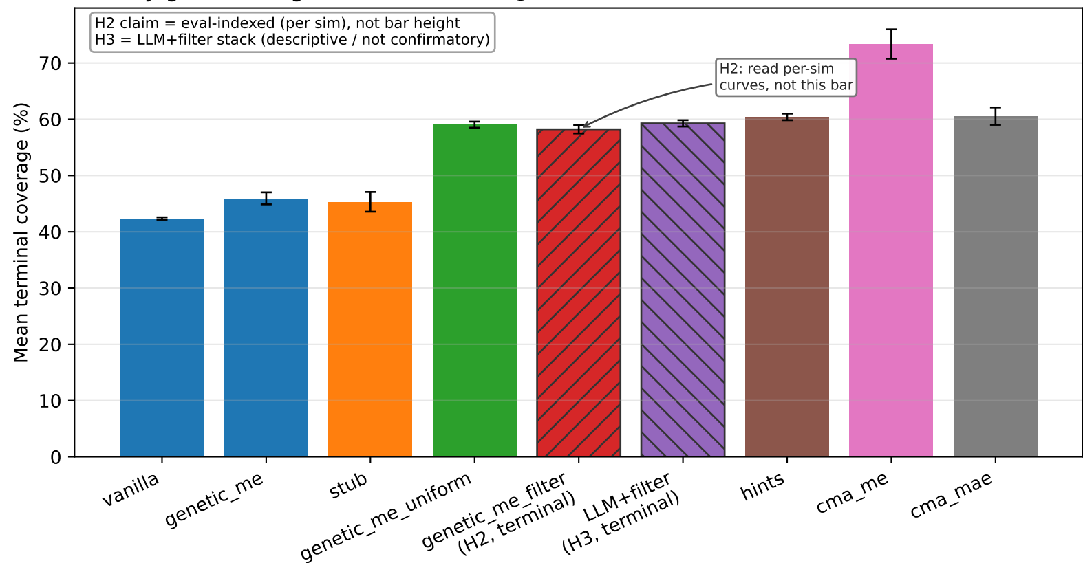
Primary-grid coverage ladder (terminal @ fixed iterations; mean \pm Student-t 95% CI; n=10)
