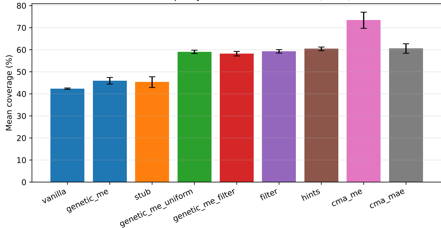
CA ladder: policy, Role-2 filter, LLM stack (n=10)
