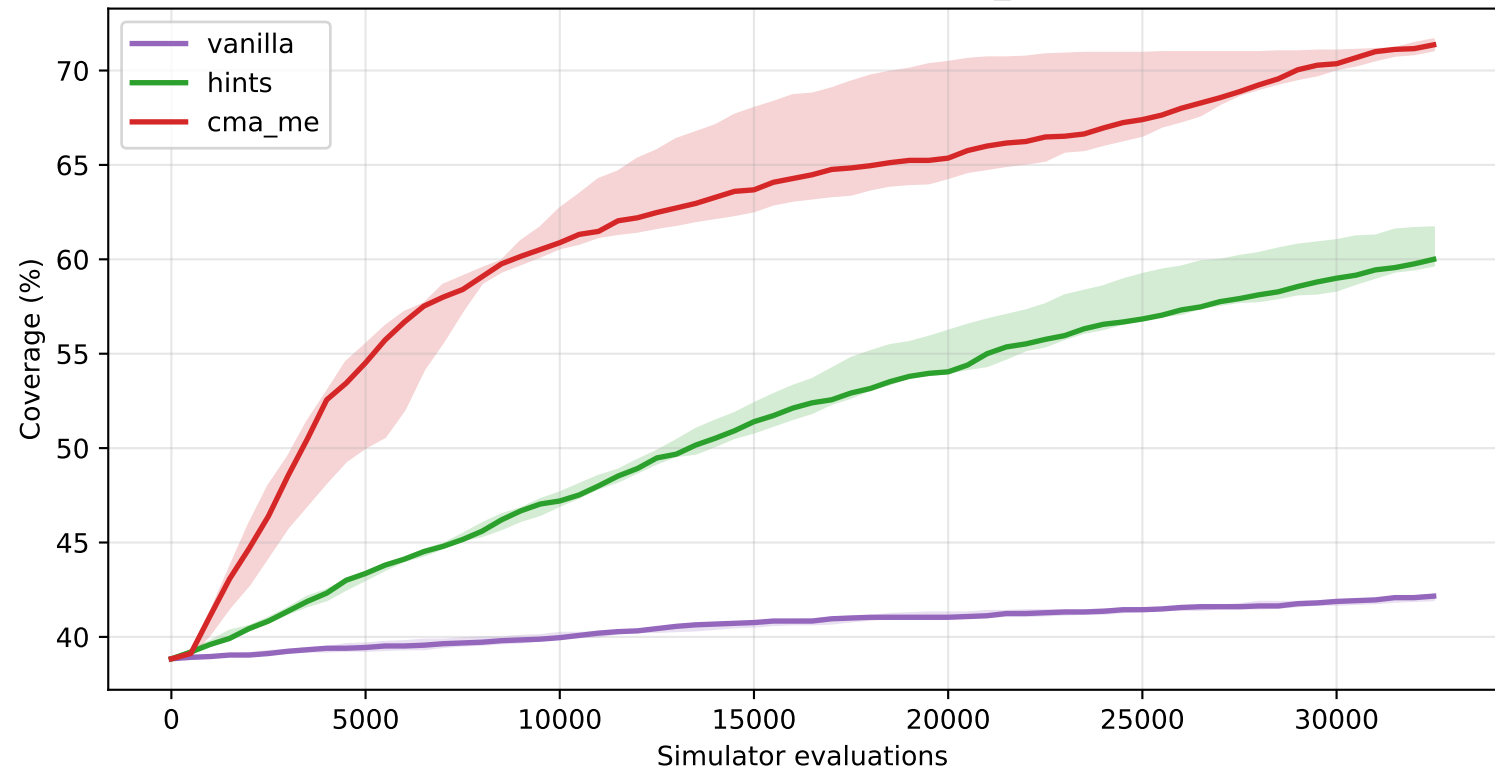
Anytime ladder: vanilla vs hints vs cma_me (n=5, IQR)
