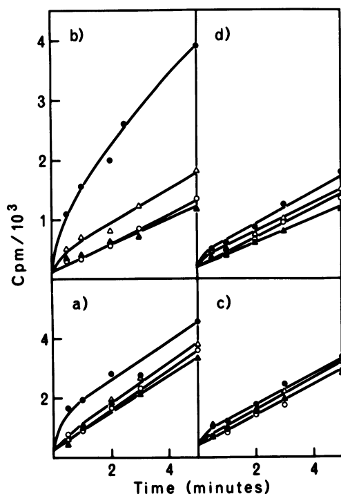
FIG. 3. Patterns of ^{14}\text{C} -tryptophan ( 10^{-5} M, 5 mCi/mmol) uptake per ml of cells at 37°C in: (a) growing W1485, (b) glucose-starved W1485, (c) growing KB3100, (d) glucose-starved KB3100. Uptake into: whole cells ( \bullet ); trichloroacetic acid-insoluble material ( \circ ); whole cells in presence of unlabeled phenylalanine 2 \times 10^{-4} M ( \Delta ); and trichloroacetic acid-insoluble material in presence of unlabeled phenylalanine, 2 \times 10^{-4} M ( \blacktriangle ). An uptake of 10^3 counts per min per ml is equivalent to 2.2 \mu\text{moles/g} (dry weight) of cells.
