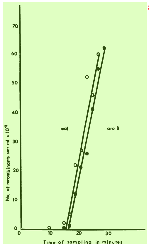
FIG. 2. Kinetics of zygote formation when the Hfr AB313 is mated with the female AB2847.
