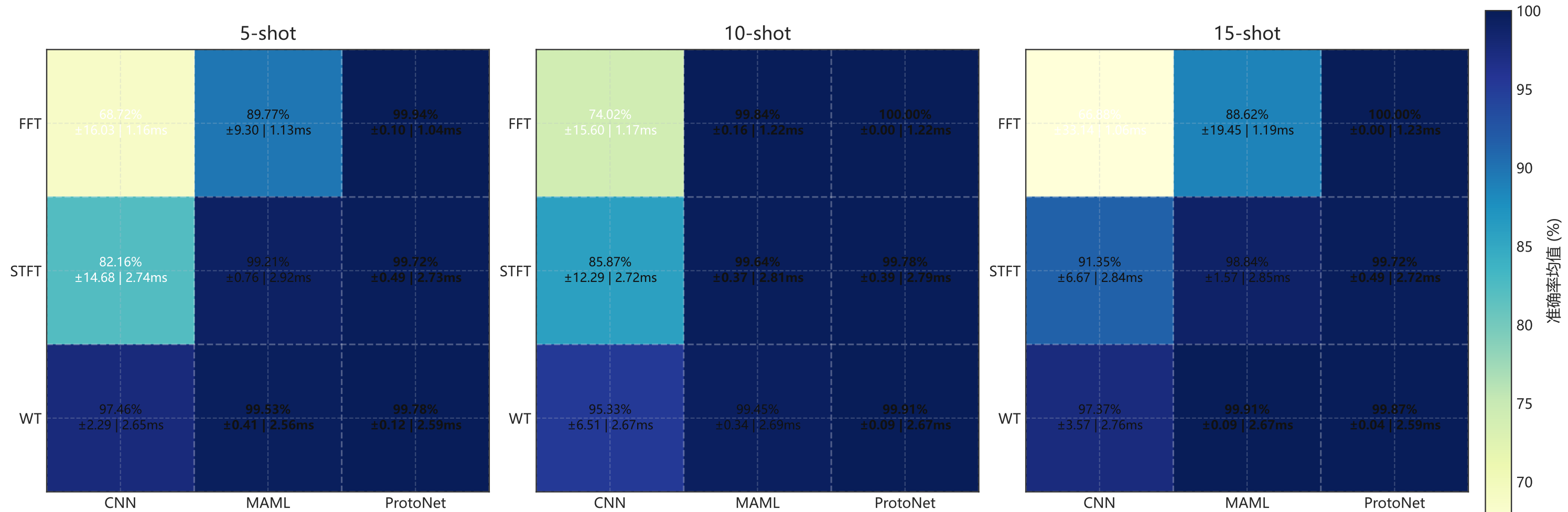
Accuracy Matrix Heatmap across Preprocessing, Model, and Shot Settings
