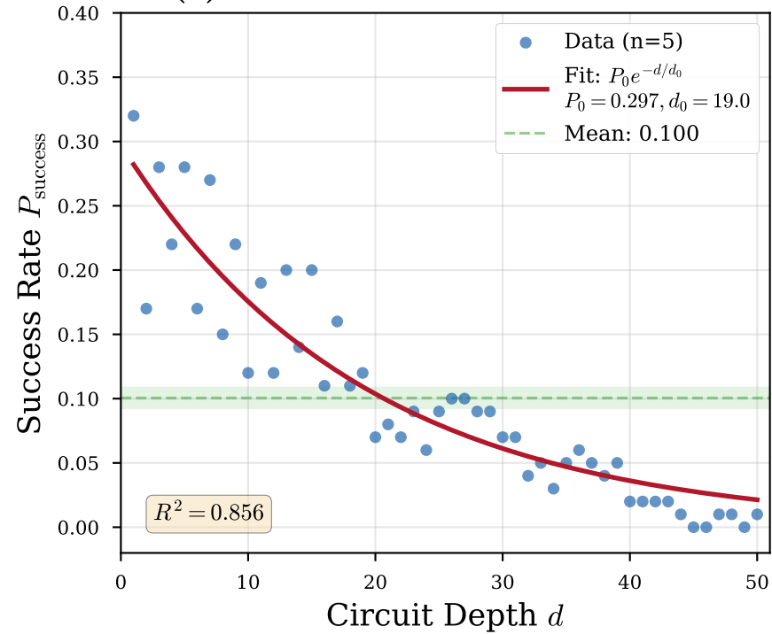
(a) Phase Transition: Success Rate
