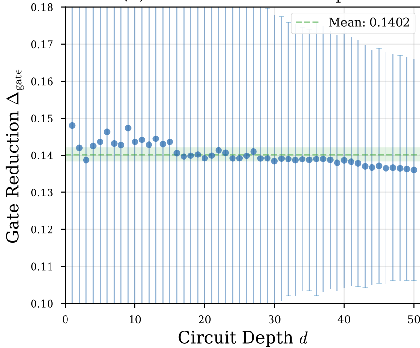
(b) Gate Reduction vs Depth
