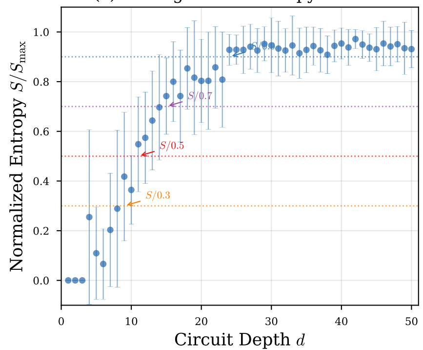
(c) Entanglement Entropy Growth
