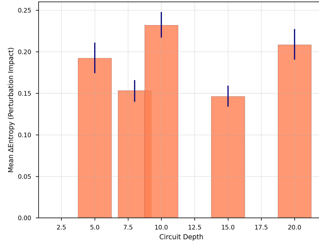
(b) Mean Perturbation Impact
