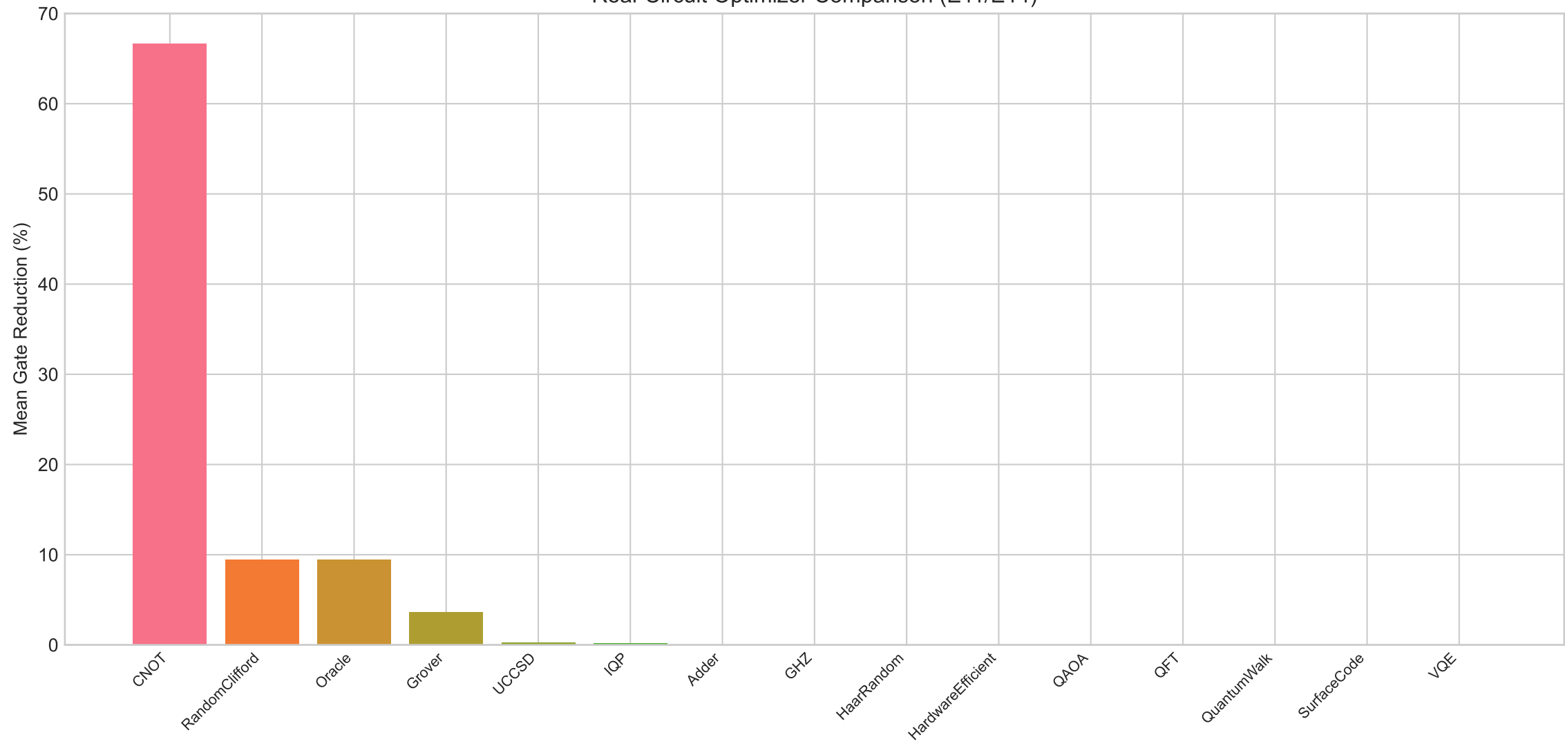
Real-Circuit Optimizer Comparison (E11/E14)
